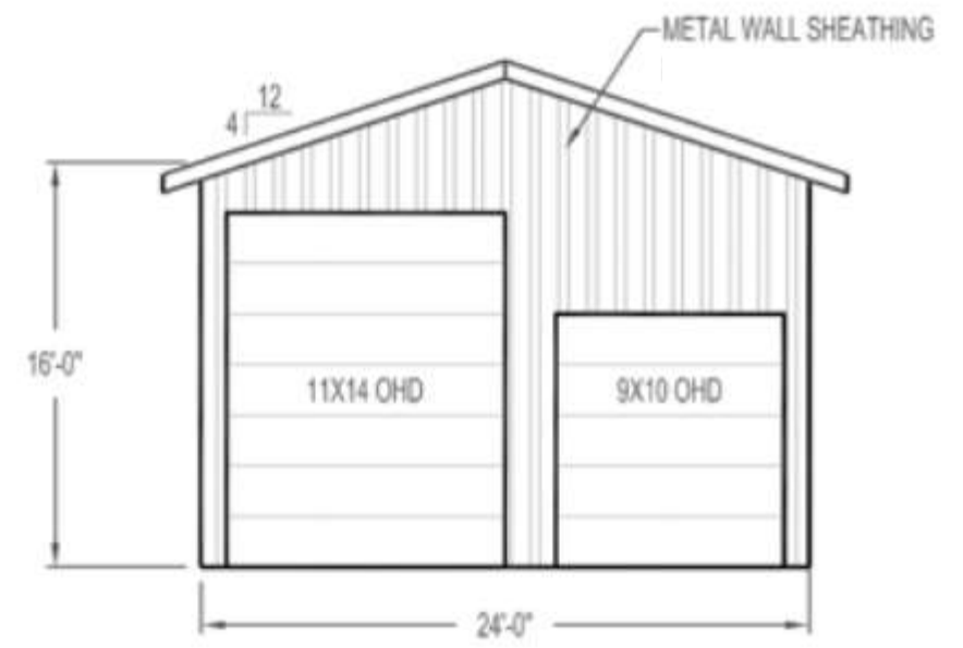
LEFT GABLE
