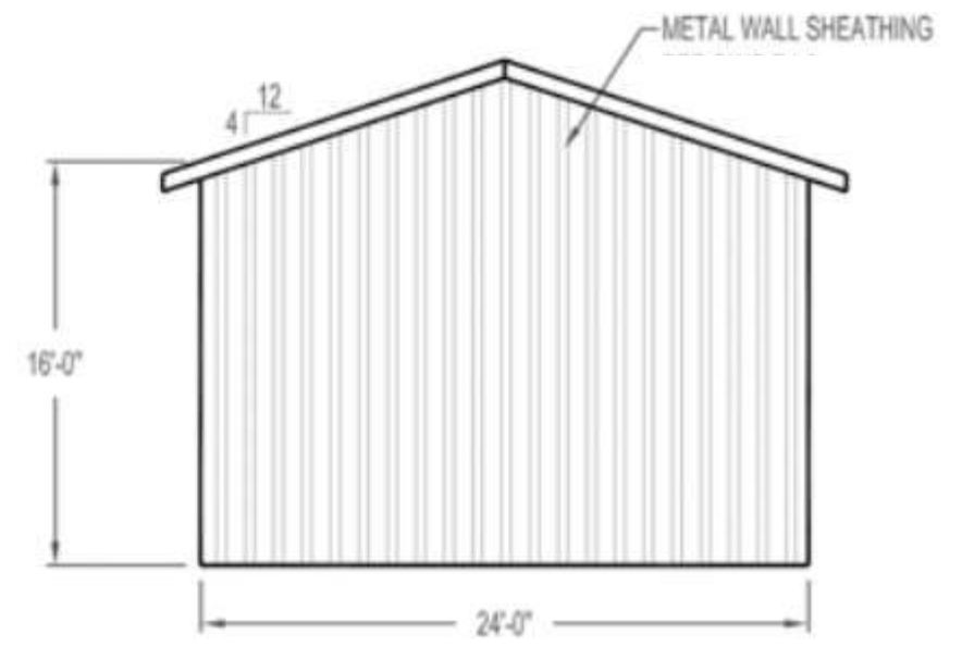
RIGHT GABLE
