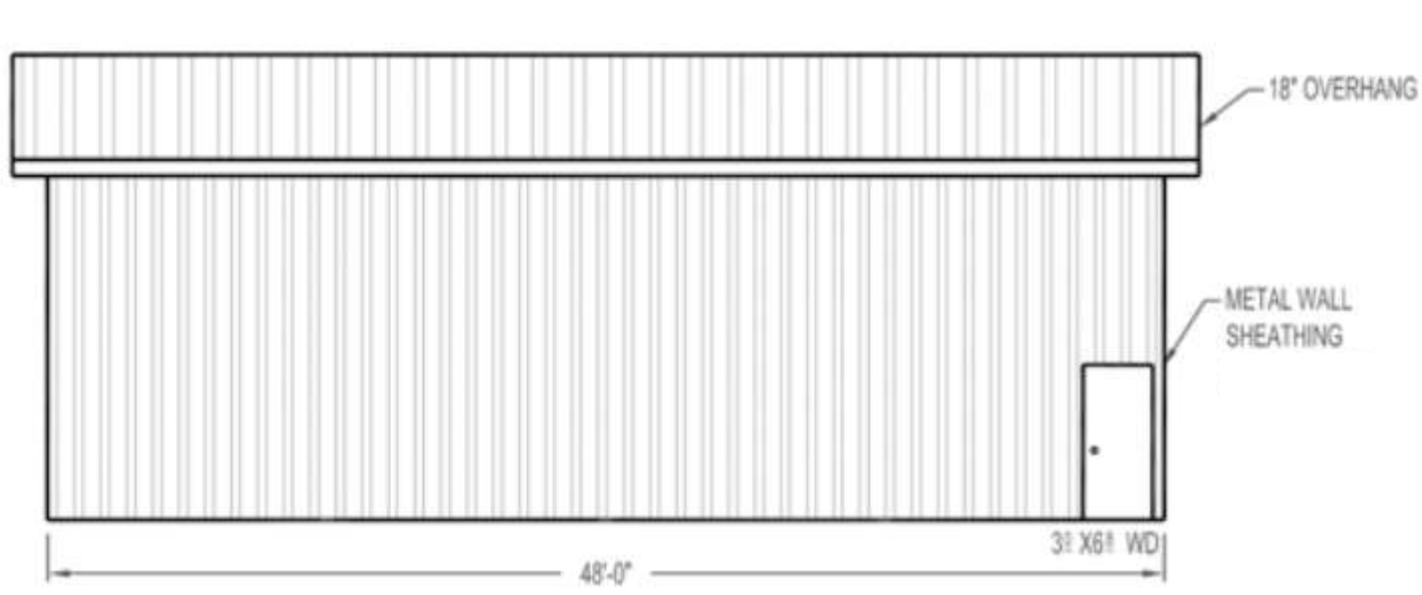
FRONT EAVE
