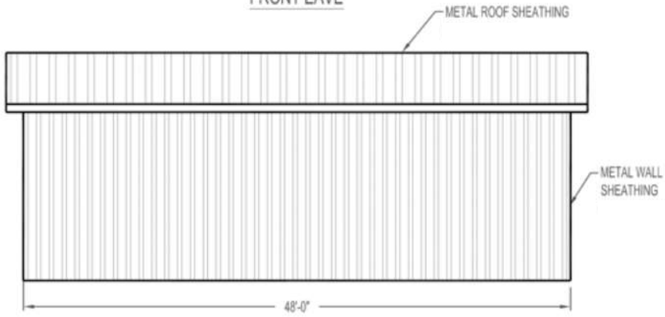
REAR EAVE
