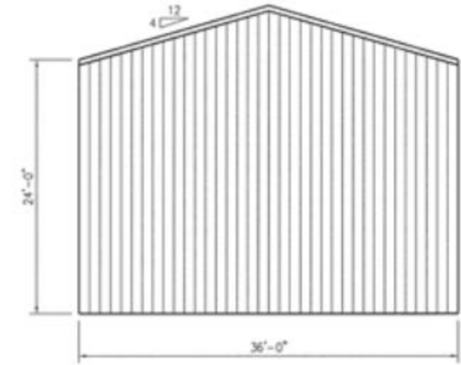
LEFT GABLE VIEW
