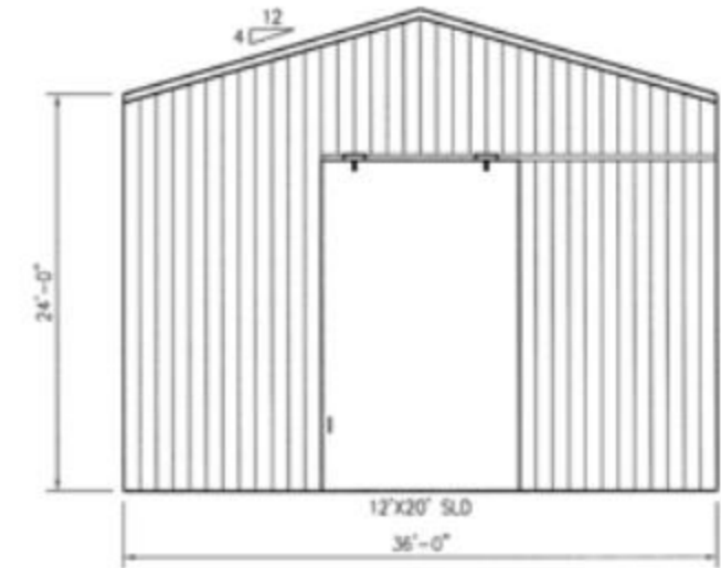
RIGHT GABLE VIEW
