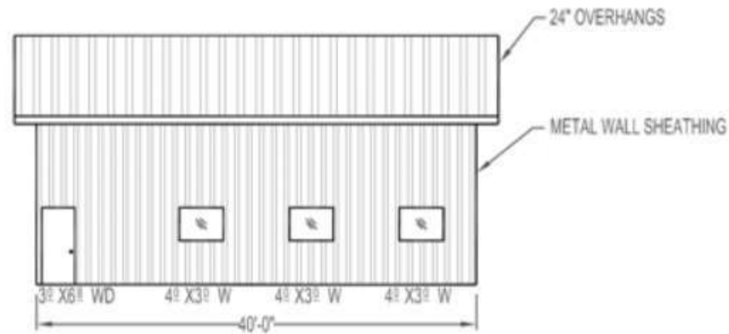
FRONT EAVE
