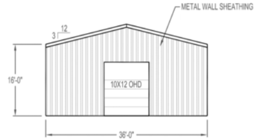
RIGHT GABLE
