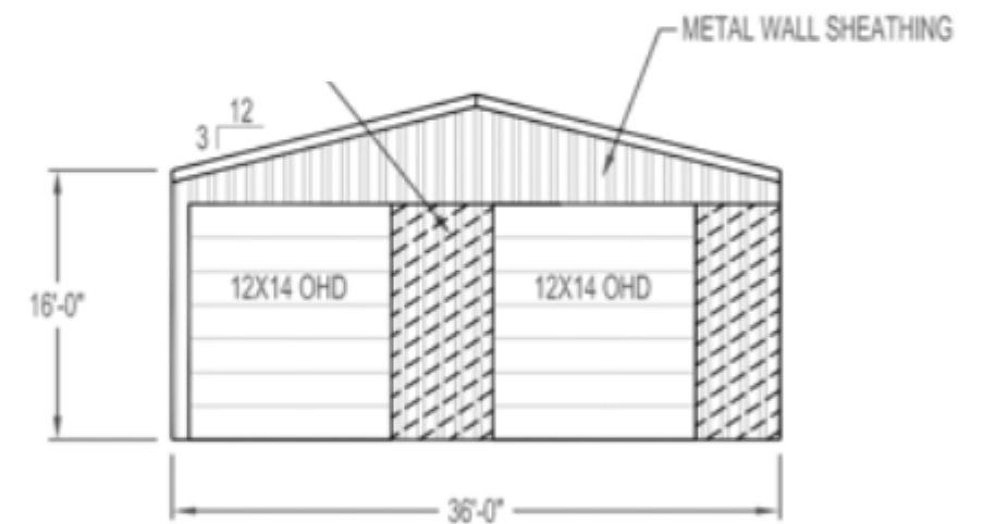
LEFT GABLE
