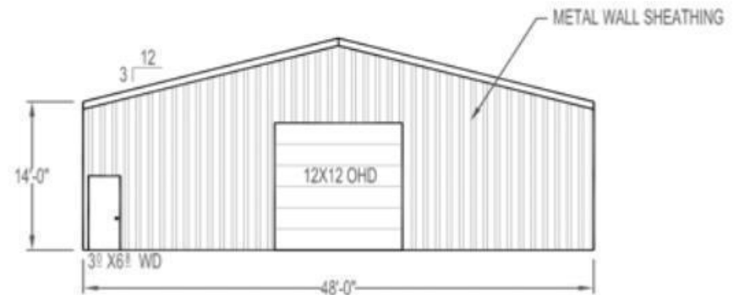
LEFT GABLE
