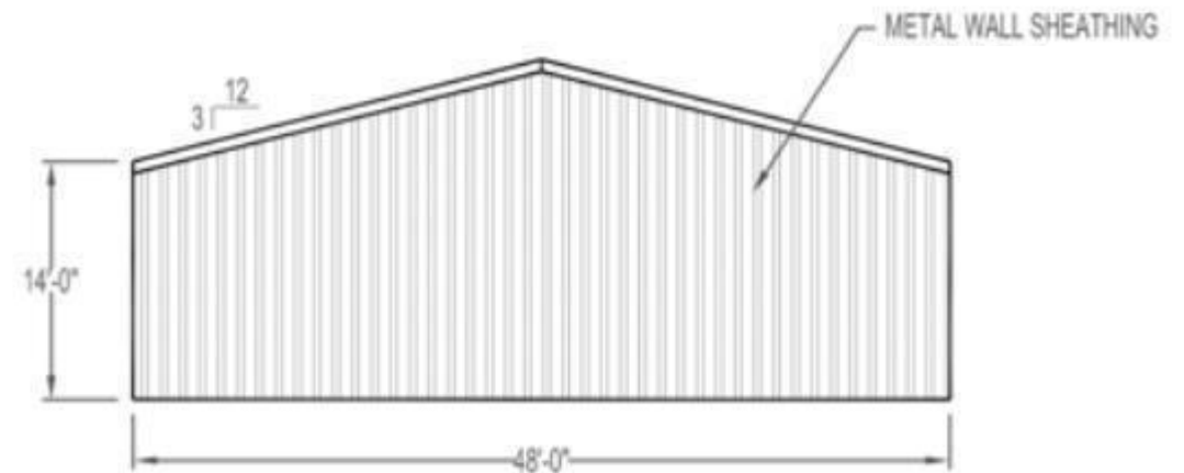
RIGHT GABLE
