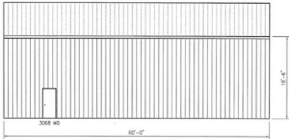
FRONT EAVE VIEW
