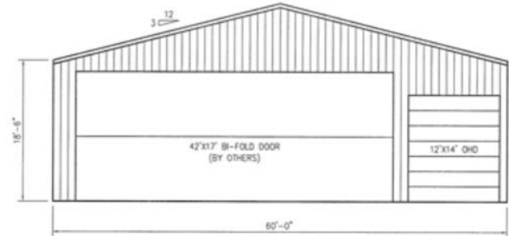
LEFT GABLE VIEW
