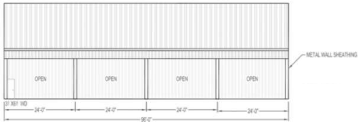
FRONT EAVE
