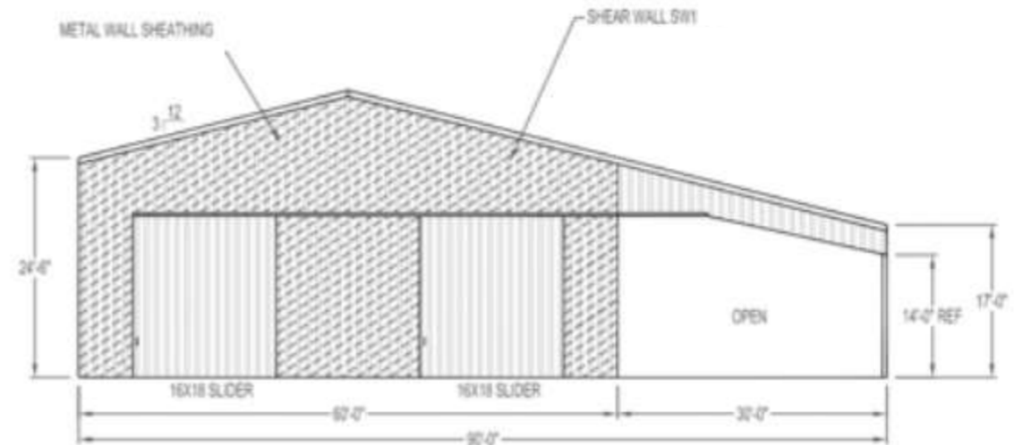
LEFT GABLE
