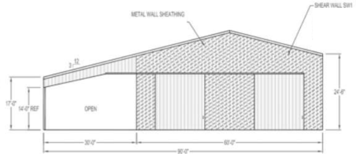
RIGHT GABLE
