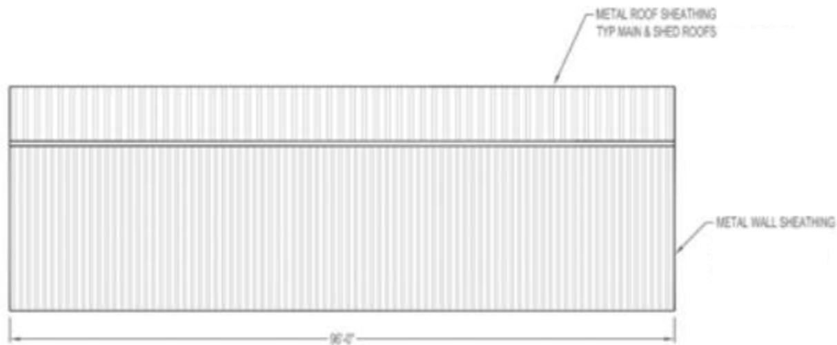
FRONT EAVE
