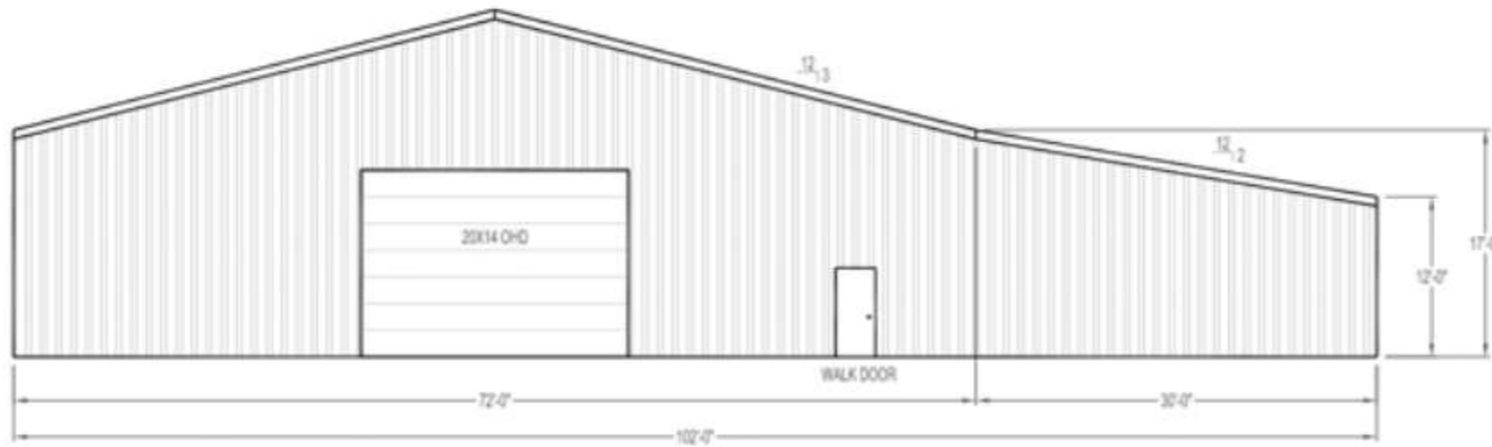
LEFT GABLE
