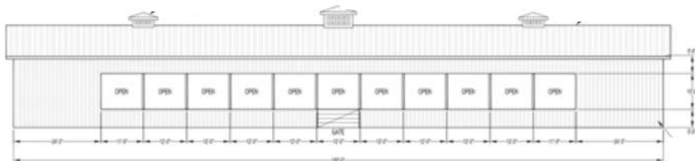
REAR EAVE
