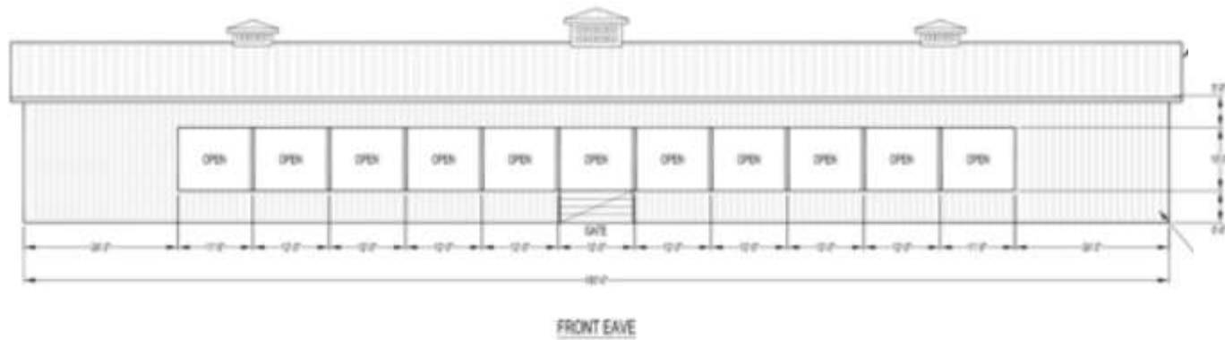
FRONT EAVE
