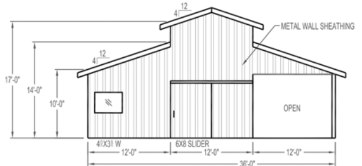
RIGHT GABLE
