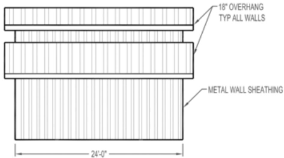
FRONT EAVE
