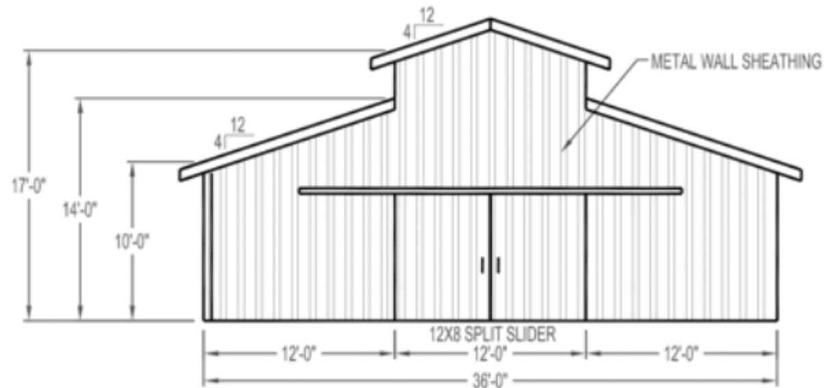
RIGHT GABLE
